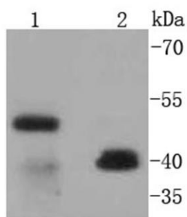
Fig. 1. Western blot analysis of CD38 on different lysates using anti-CD38 antibody at 1/1,000 dilution. Positive control: Lane 1: THP-1; Lane 2: Raji
